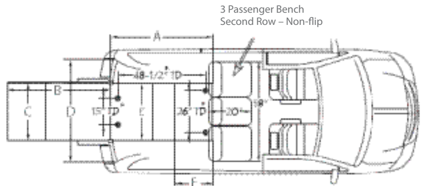
1 Wheelchair Configuration
